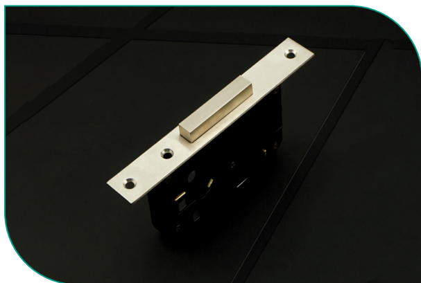
| Deadlock
